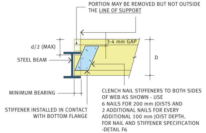
DETAIL F8
