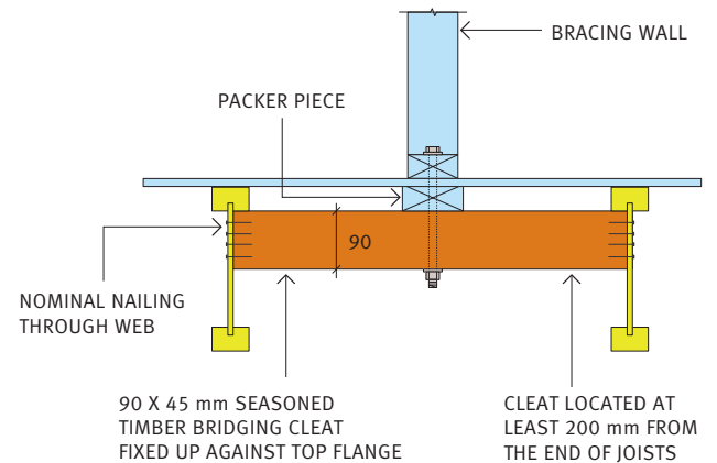
DETAIL F9
